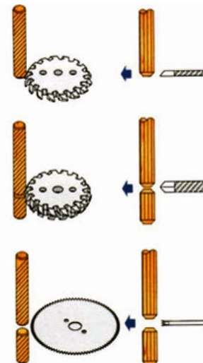
Dowel chamfering & cutting
