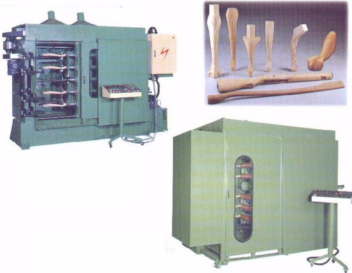
CL-1006 Auto Copy Lathe CL-1006ST Auto Copy Lathe with Sander
