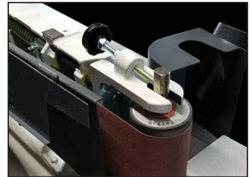
EASY ADJUSTMENT FOR BELT TRACKING
