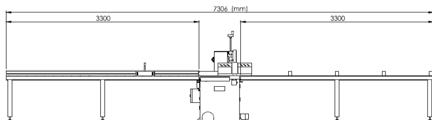
Optional In & Out Feed roller Table
