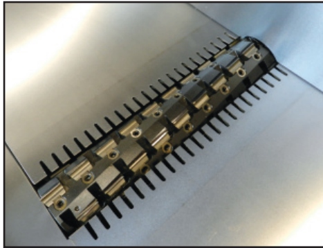
Spiral Insert Knife Cutterhead Equipped with a spiral insert knife cutterhead with 2-sided 30x12x1.5mm replaceable insert knives which provides a superior finish & ultra-quiet operation.
