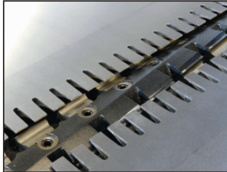
Noise Reduction Table Lips Both infeed and outfeed tables are equipped with unique noise reduction table lips which are contoured close to the cutterhead for safe and quiet operation. Also equipped with a rabbeting ledge on the infeed table with a Max. Depth of 3/4"
